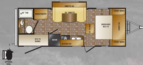
ST24RB 24" LCD TV STD.
