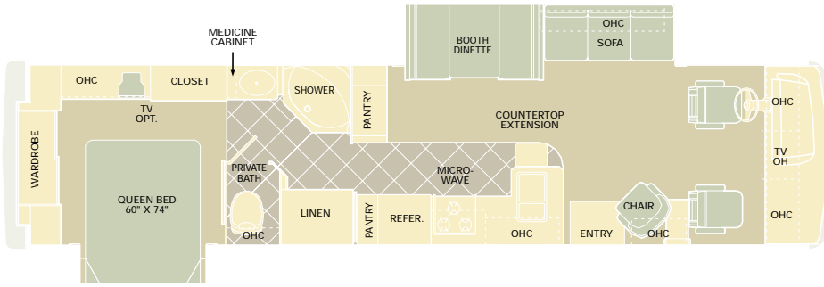
MODEL | 36WDD
