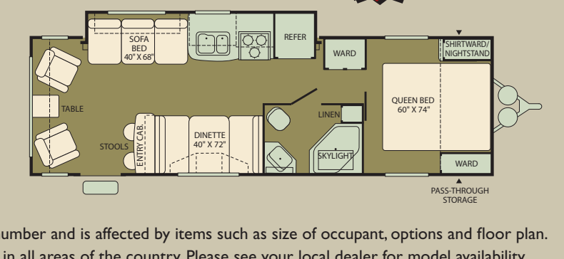
280RLSS Single Slide-Out • Sleeps 5-6* NEW FLOOR PLAN
