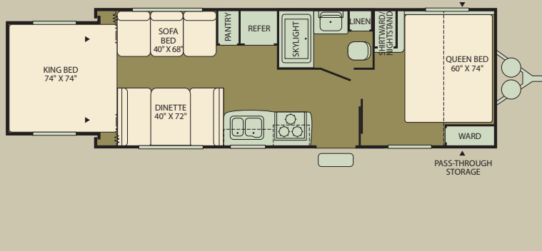
260RKSS Single Slide-Out • Sleeps 5-6* NEW FLOOR PLAN
