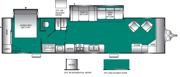
39BHDS Sleeps 9 - 10*, Double Slide-Out
