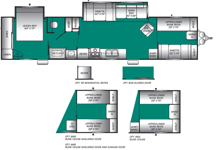
39BHDS Sleeps 9 - 10*, Double Slide-Out
