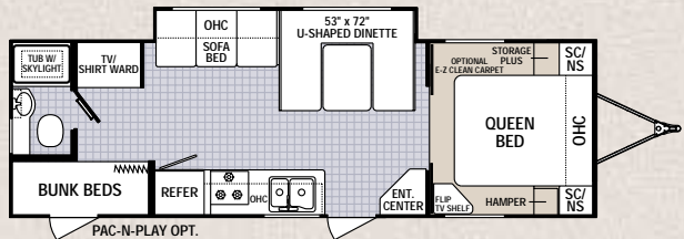
30BH-SL (available with Pac-n-Play storage option)
